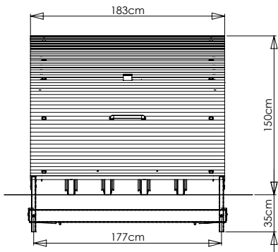
Type 1.8 (4 bikes)
